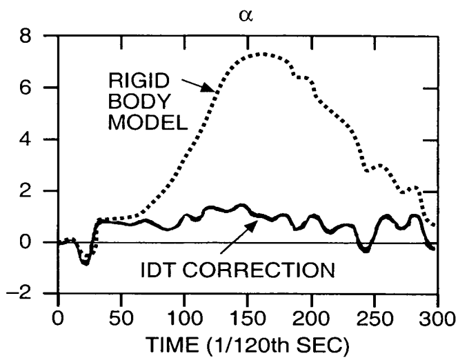
ORIENTATION (deg) FIG._17A
